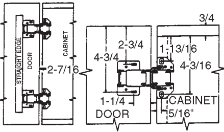
3/4" OVERLAY
