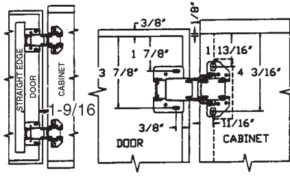
FULL INSET
